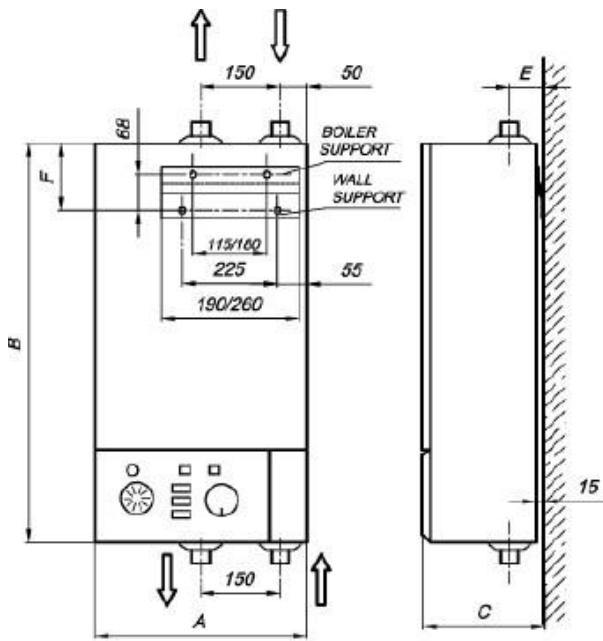
BOILERS 4,5 - 24 kW
