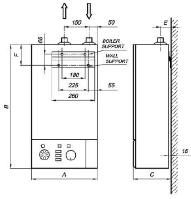
BOILERS 28 - 96 kW
